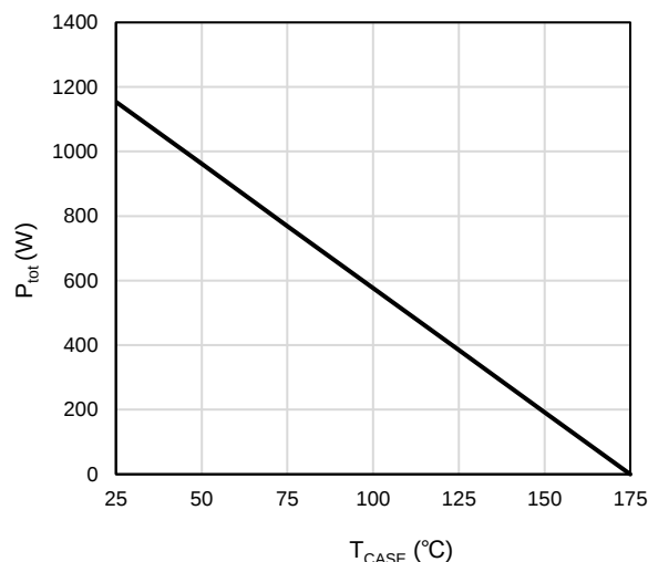
Figure 2: Power De-rating
